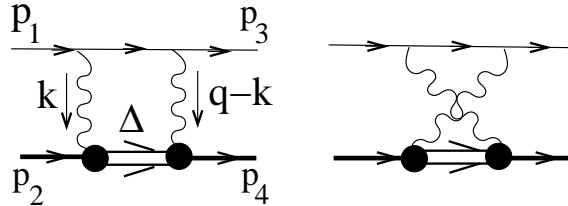
FIG. 1: Two-photon exchange box and crossed-box graphs for electron-proton scattering with a \Delta intermediate state, calculated in the present letter.
