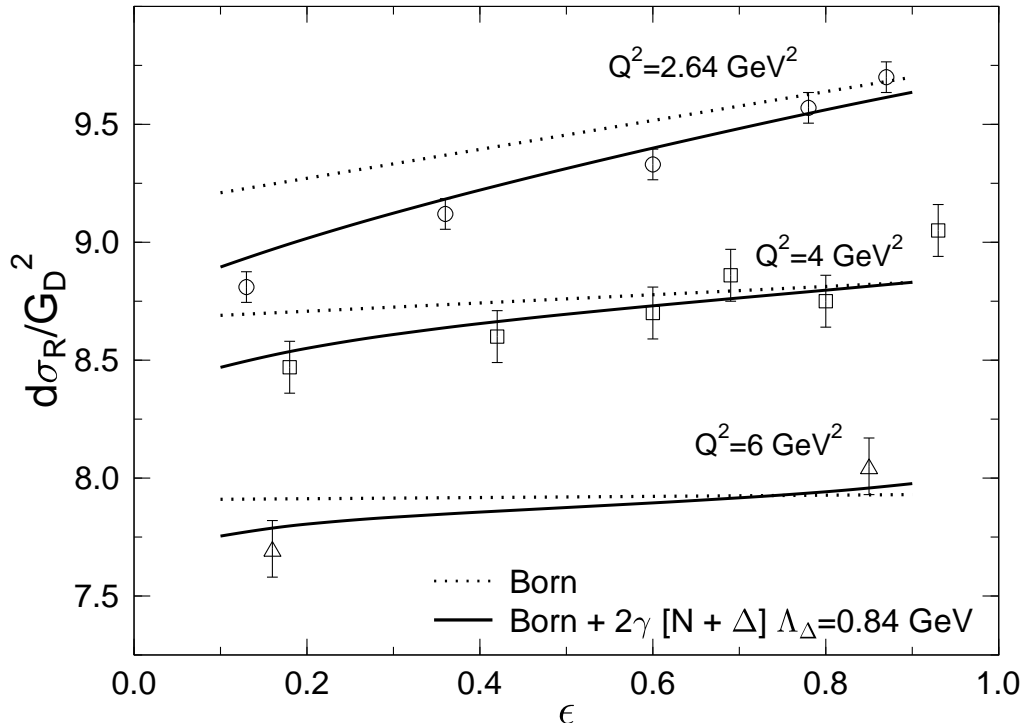
FIG. 3: Effect of adding the two-photon exchange (with the indicated choice of the \gamma N\Delta form factor) to the Born cross section, the latter evaluated with the nucleon form factors from the PT experiment [3, 4]. The reduced cross section is scaled as described in the text. The curves for Q^2 = 2.64, 4 and 6 \text{ GeV}^2 have been shifted vertically by -0.04, +0.04 and +0.09 , respectively. The data points at three fixed momentum transfers are taken from Refs. [1, 2].
